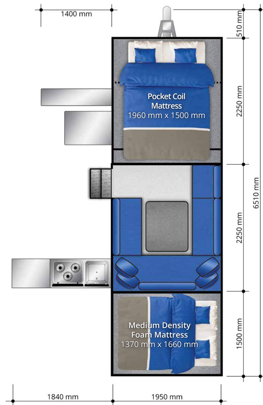
DrifterII Floor Plan (Top View)
