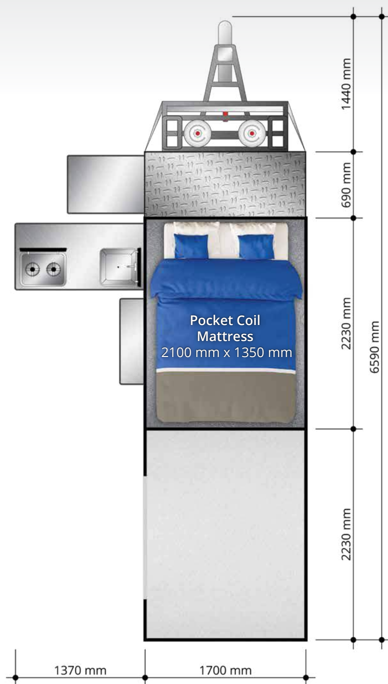
Brumby Floor Plan (Top View)
