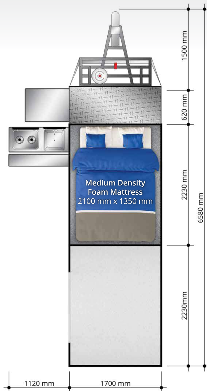
Explorer Floor Plan (Top View)
