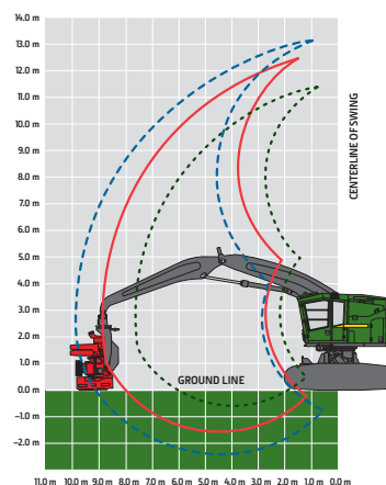
859MH Tracked Harvester
